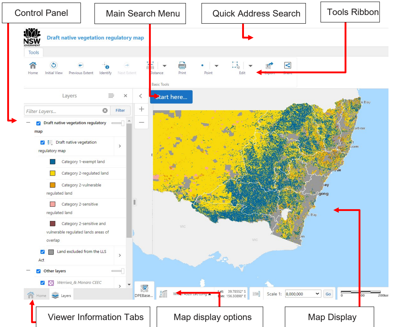
Figure 1 Home panel
