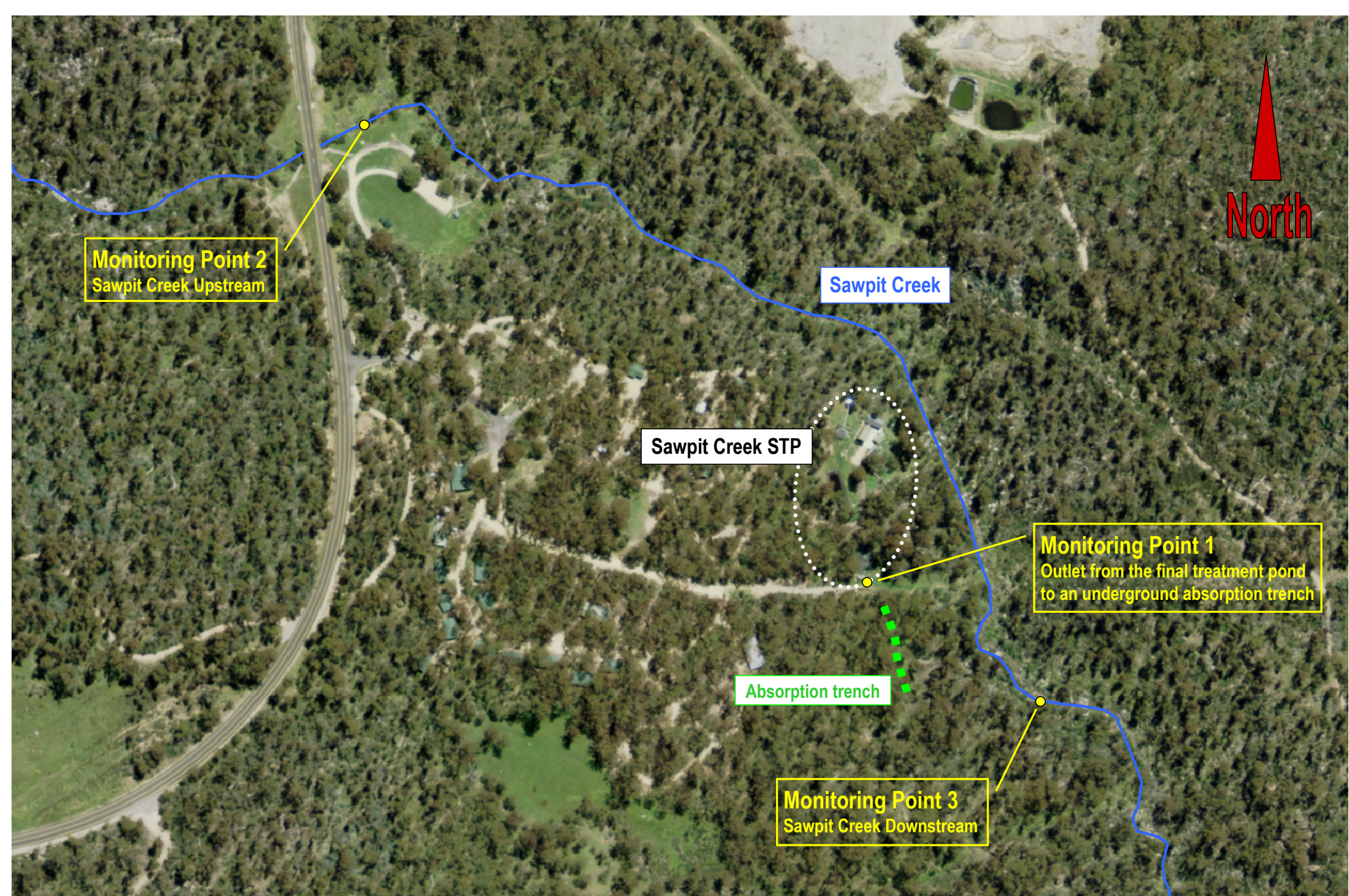
Sawpit Creek Sewage Treatment Plant (EPL No. 447) Location of monitoring points
