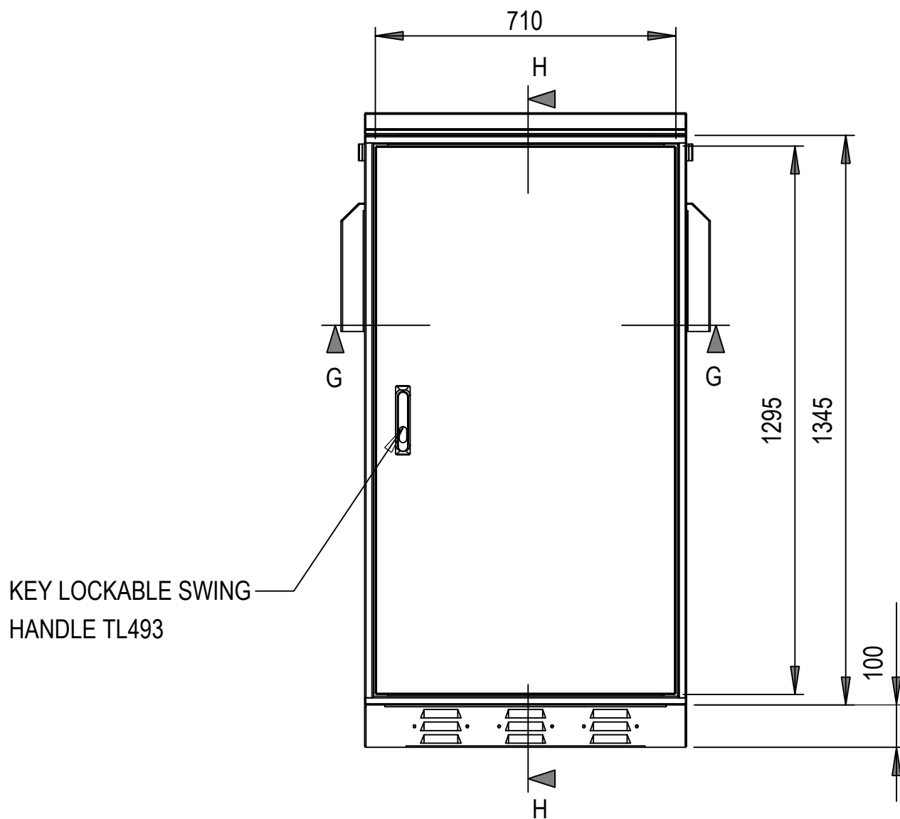
FRONT VIEW
