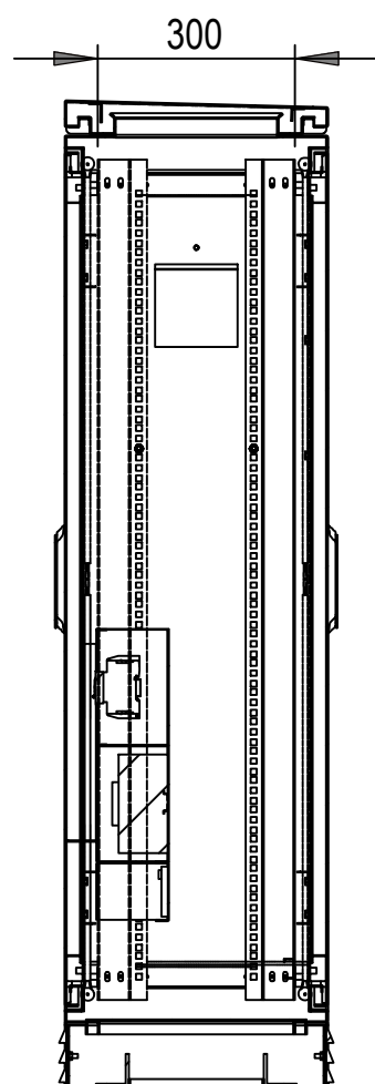
SECTION H-H
