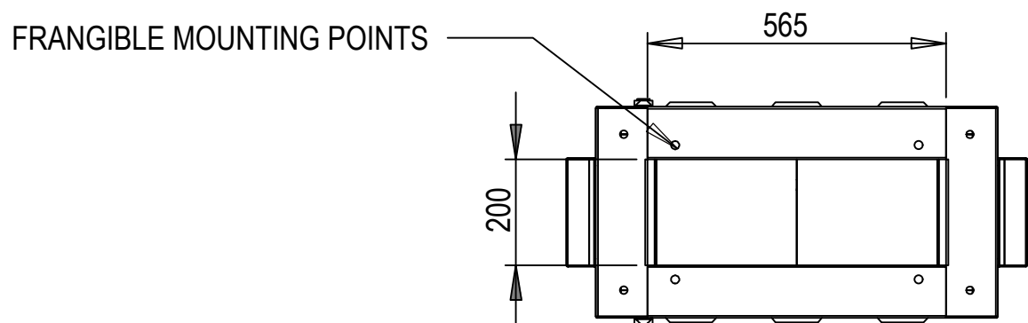
BOTTOM VIEW
